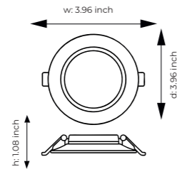
D: 100.5 mm H: 27.5 mm W: 100.5 mm Min. 75 mm Maks. 95 mm 2.95 inch 3.74 inch
